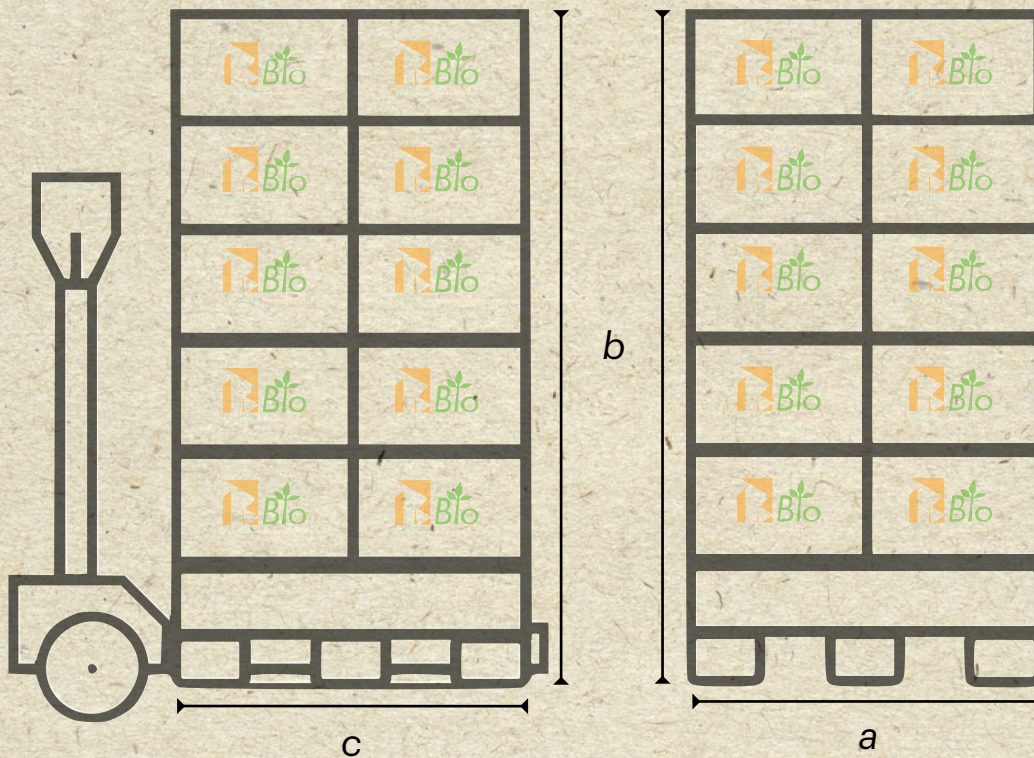
Lateral view
